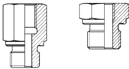
Ri- BSPP Male x Female
